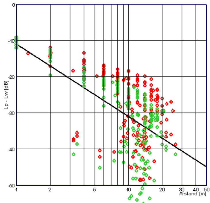
Figure 6. Absalon School. Sound propagation as function of distance before (red) and after (green) acoustical treatment in all the open areas. The straight line represents free field conditions.
