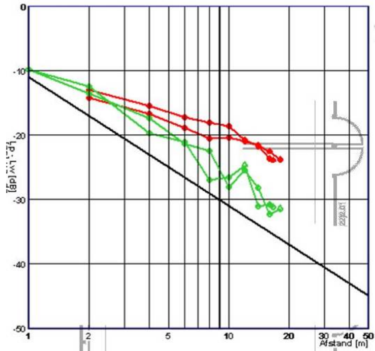
Figure 5. Absalon School. Sound propagation along measurement paths before (red) and after (green) acoustical treatment in one of the open near-areas. The straight line represents free field conditions.
